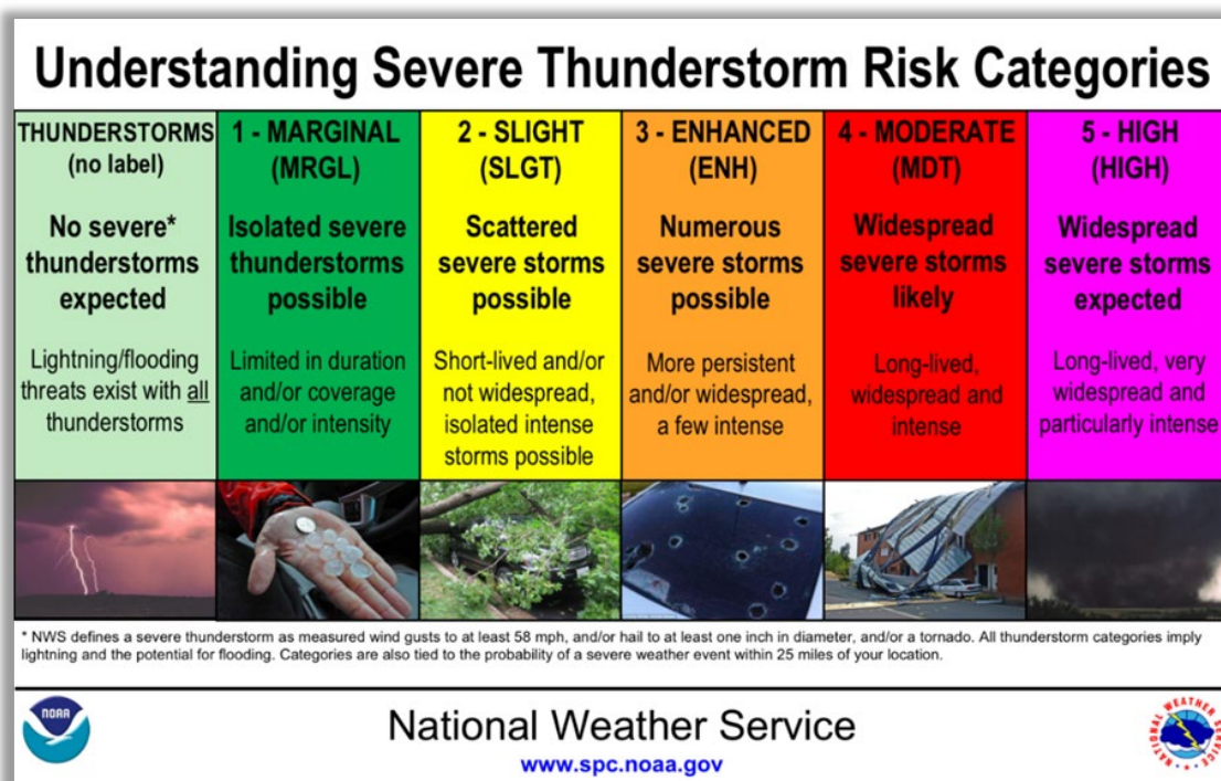
Figure 5.4.1-3. Thunderstorm Risk
